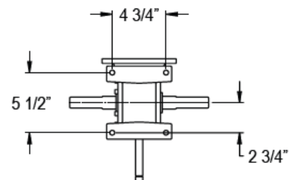
MOUNTING DIMENSIONS
