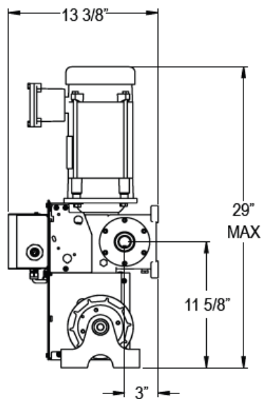
GCL-GH NEMA 7/9 OPERATOR 1/2 - 1 HP
