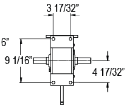
MOUNTING DIMENSIONS
