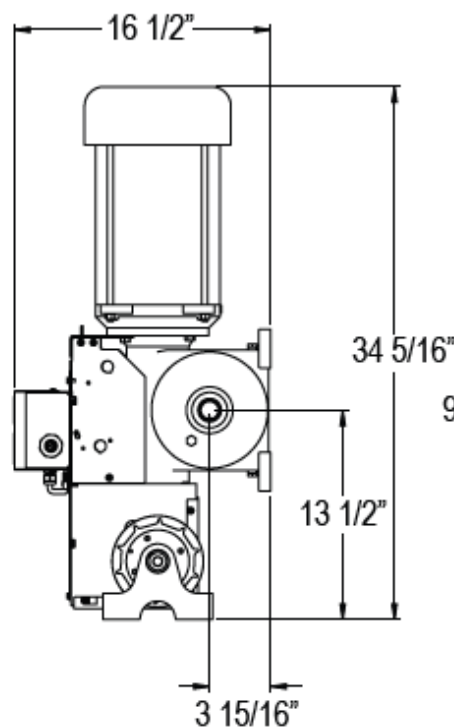
GCL-GH NEMA 7/9 OPERATOR 3 HP
